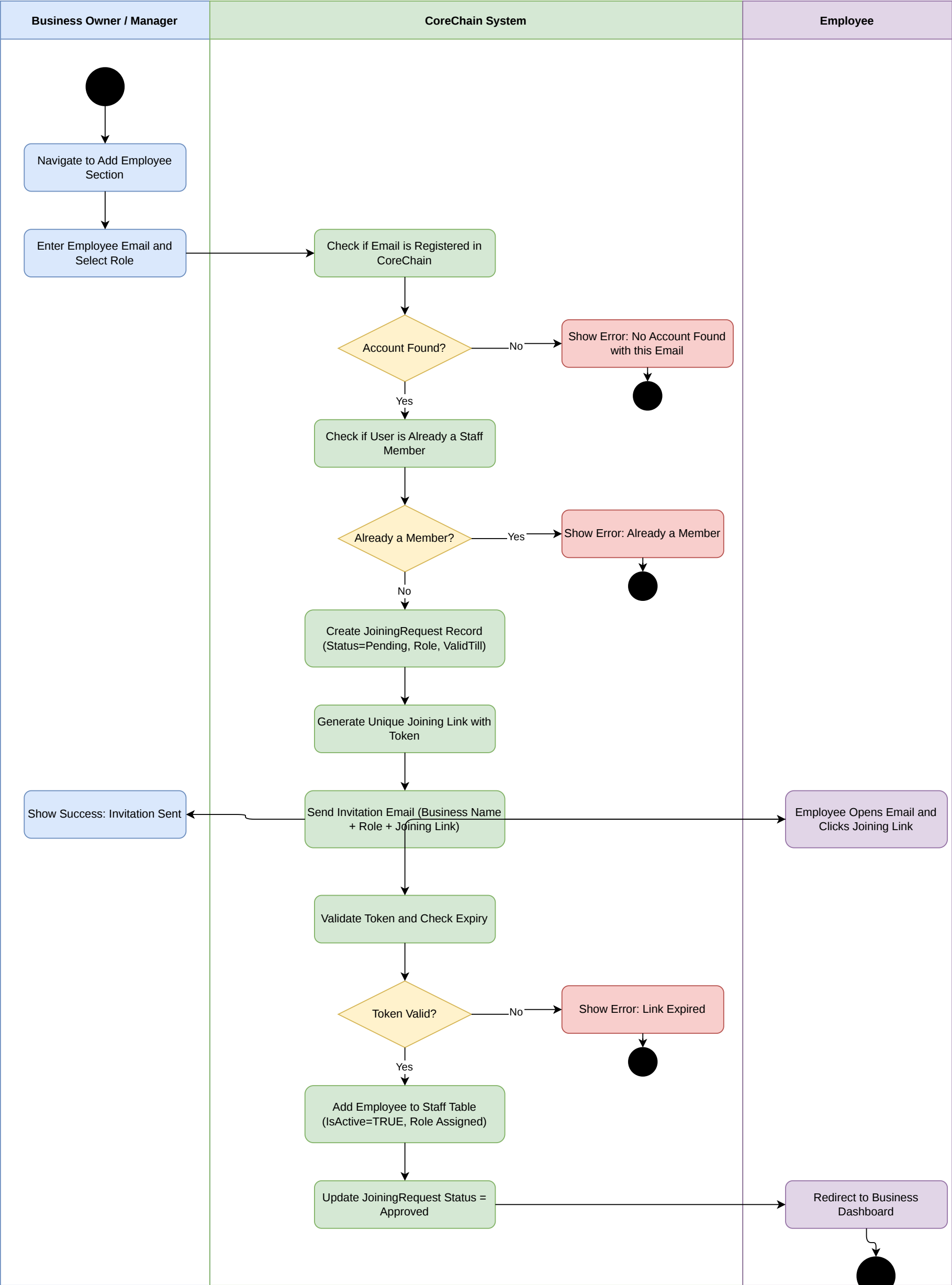
Activity Diagram: Employee Invitation and Onboarding — CoreChain
